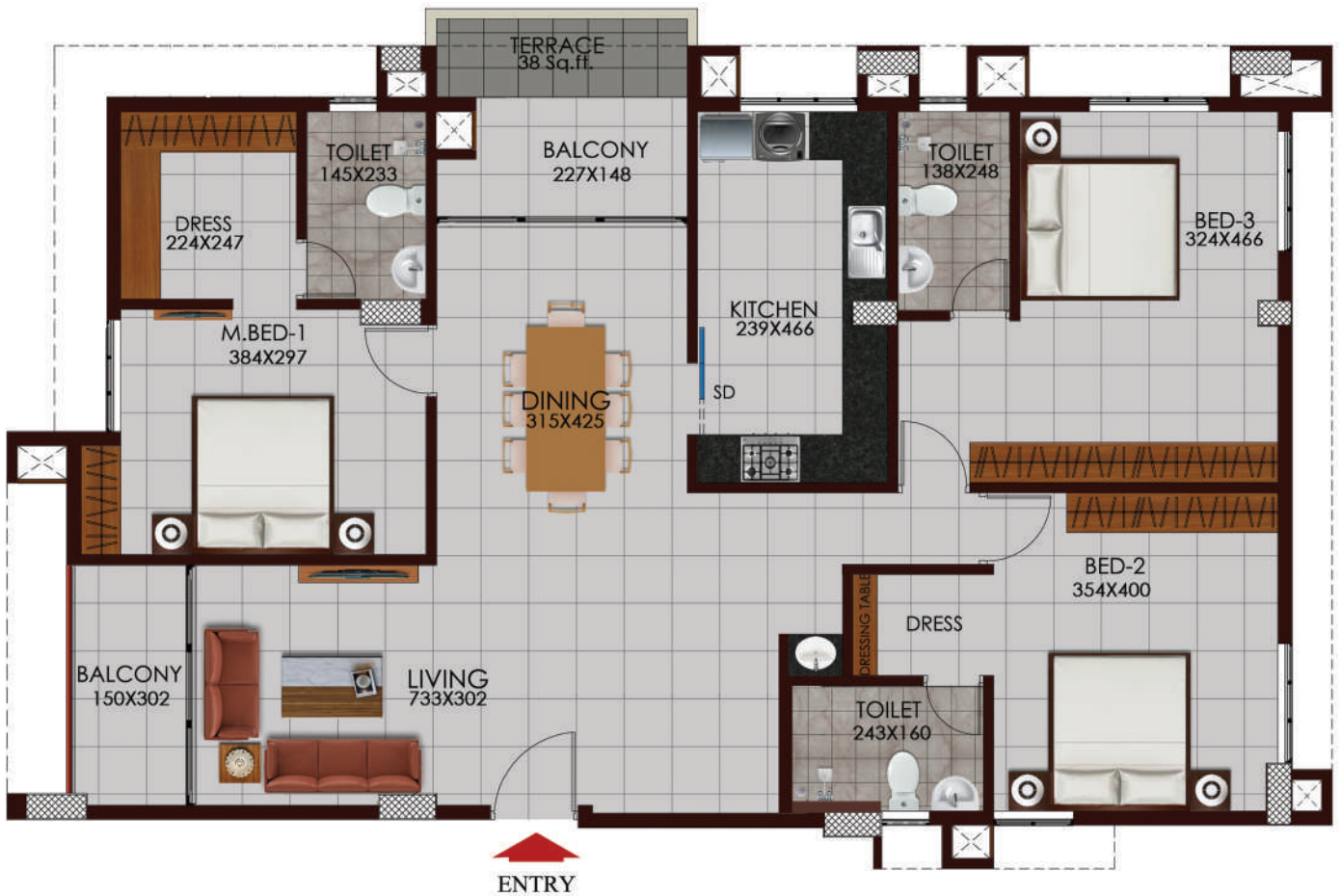
KEY PLAN
